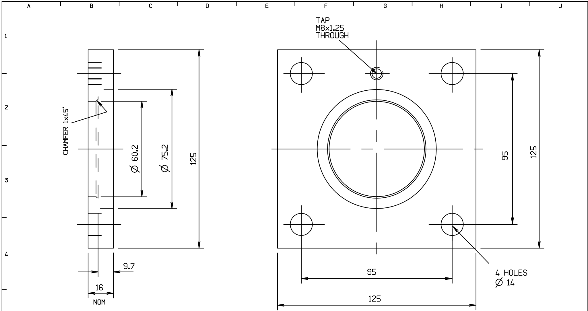
MILD STEEL RETAINING PLATE
